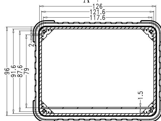
SEC B-B
