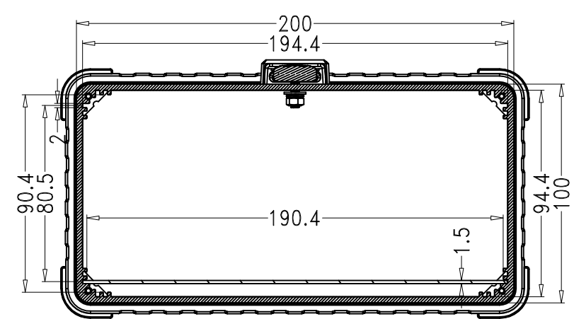
SEC B-B
