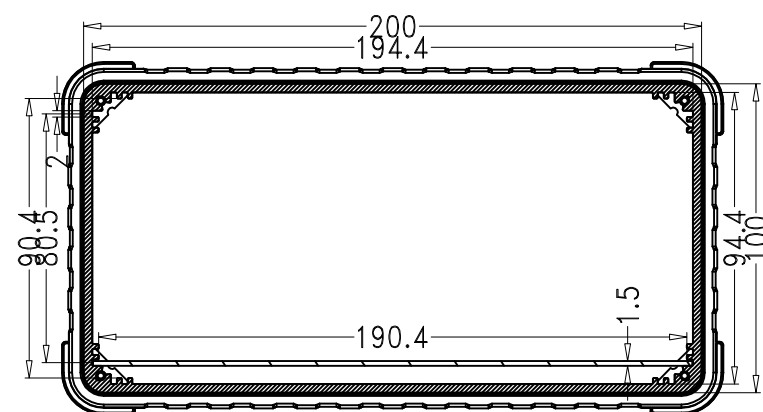
SEC B-B
