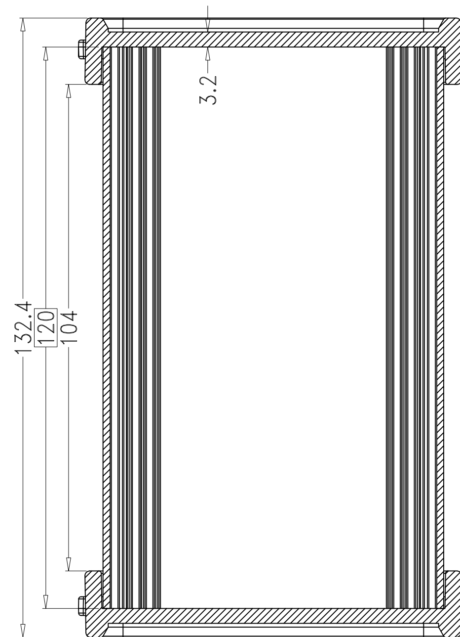
SEC B-B
