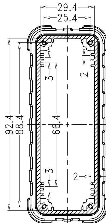
SEC B-B
