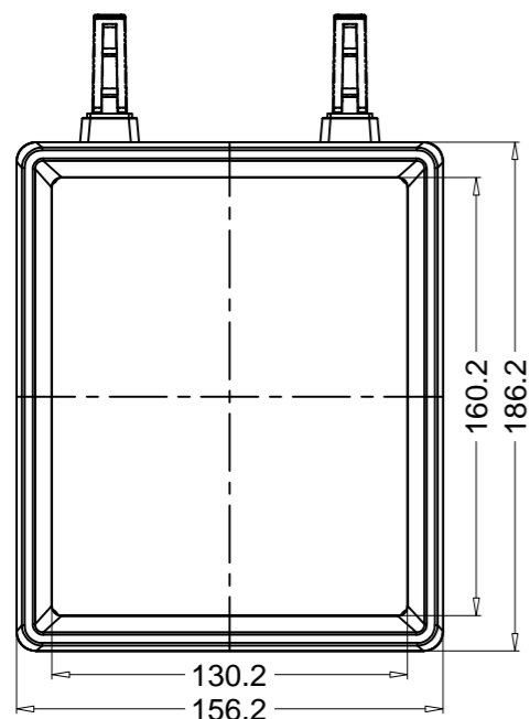
G VIEW
