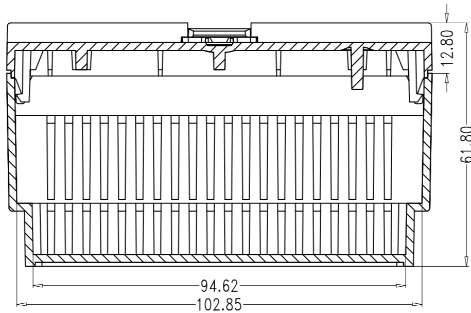
SEC B-B
