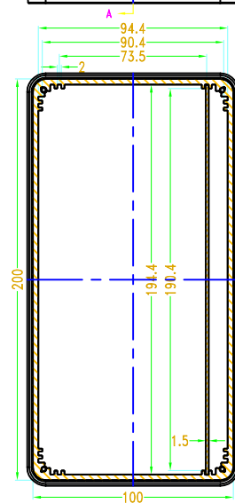
SEC B-B
