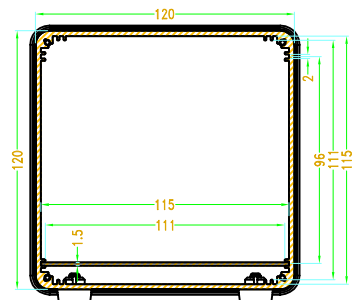
SEC B-B
