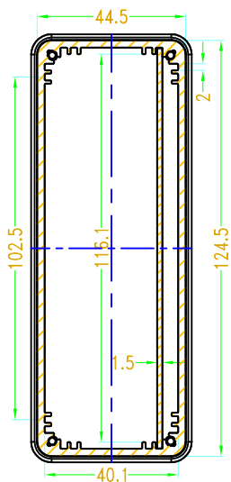
SEC B-B
