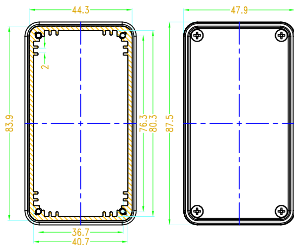
SEC B-B
