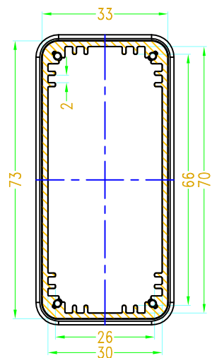
SEC B-B
