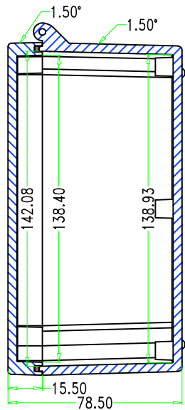
SEC B-B
