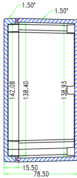
SEC B-B
