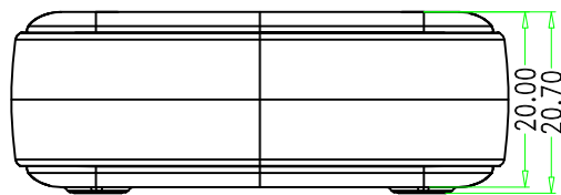
SEC B-B
