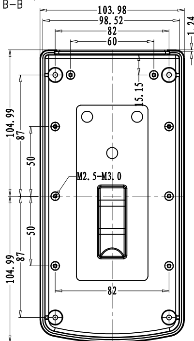
SEC B-B
