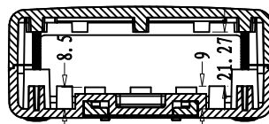
SEC B-B
