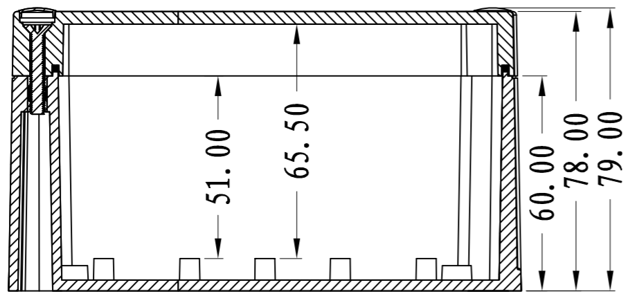
SEC B-B
