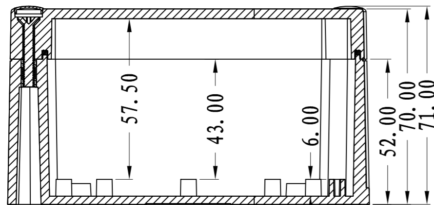
SEC B-B
