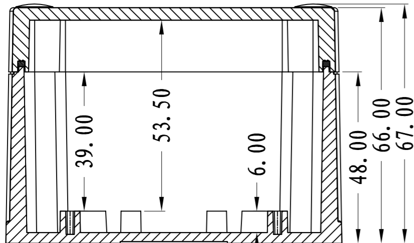
SEC B-B
