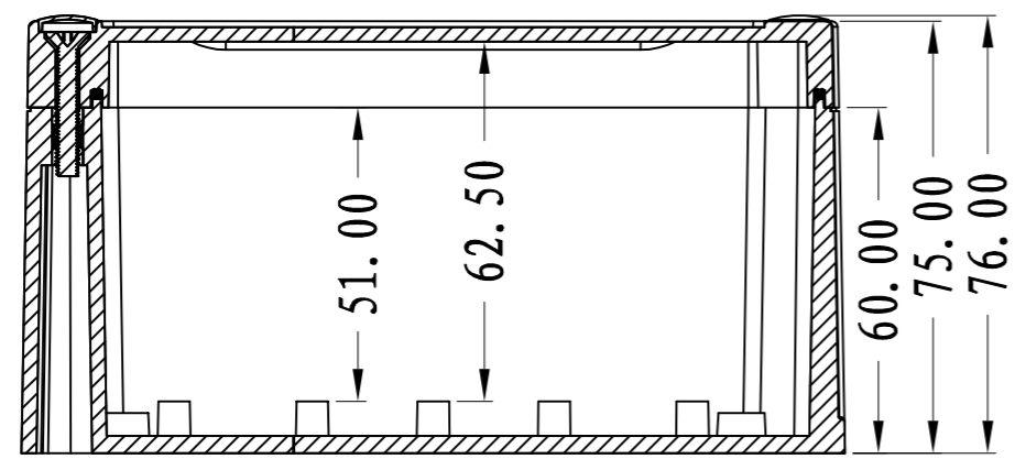
SEC B-B
