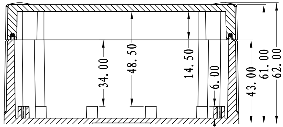
SEC B-B
