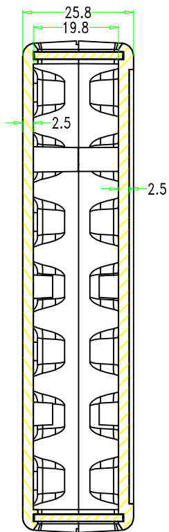
SEC B-B
