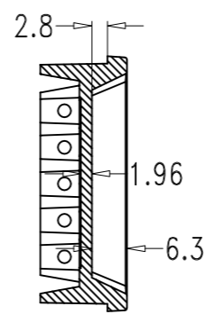
SEC B-B
