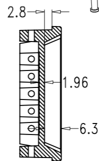
SEC B-B
