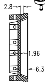
SEC B-B
