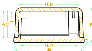
SEC B-B
