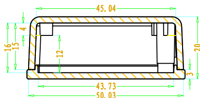
SEC B-B
