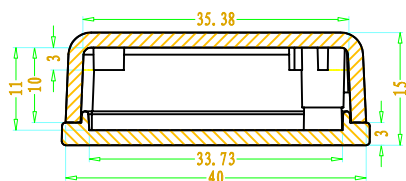
SEC B-B
