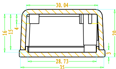
SEC B-B
